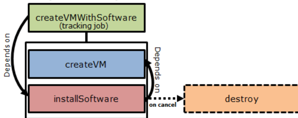
Sample Cloud Workflow (submit order)
