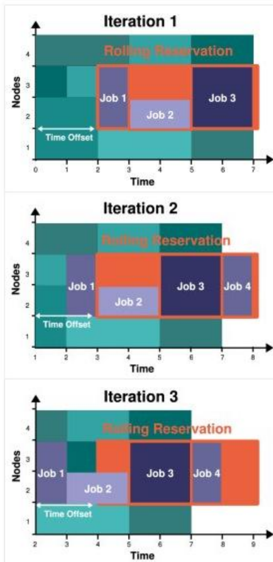
Example 9: Rollback Reservations
