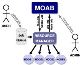
Image 14-1: Traditional TORQUE/Moab setup
