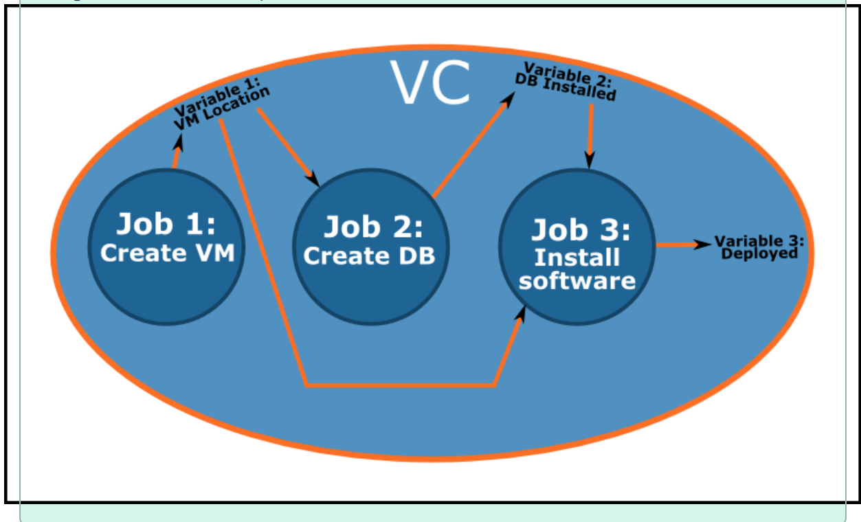
Image 24-2: Workflow example
