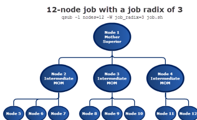
Image 5-1: Job radix example
